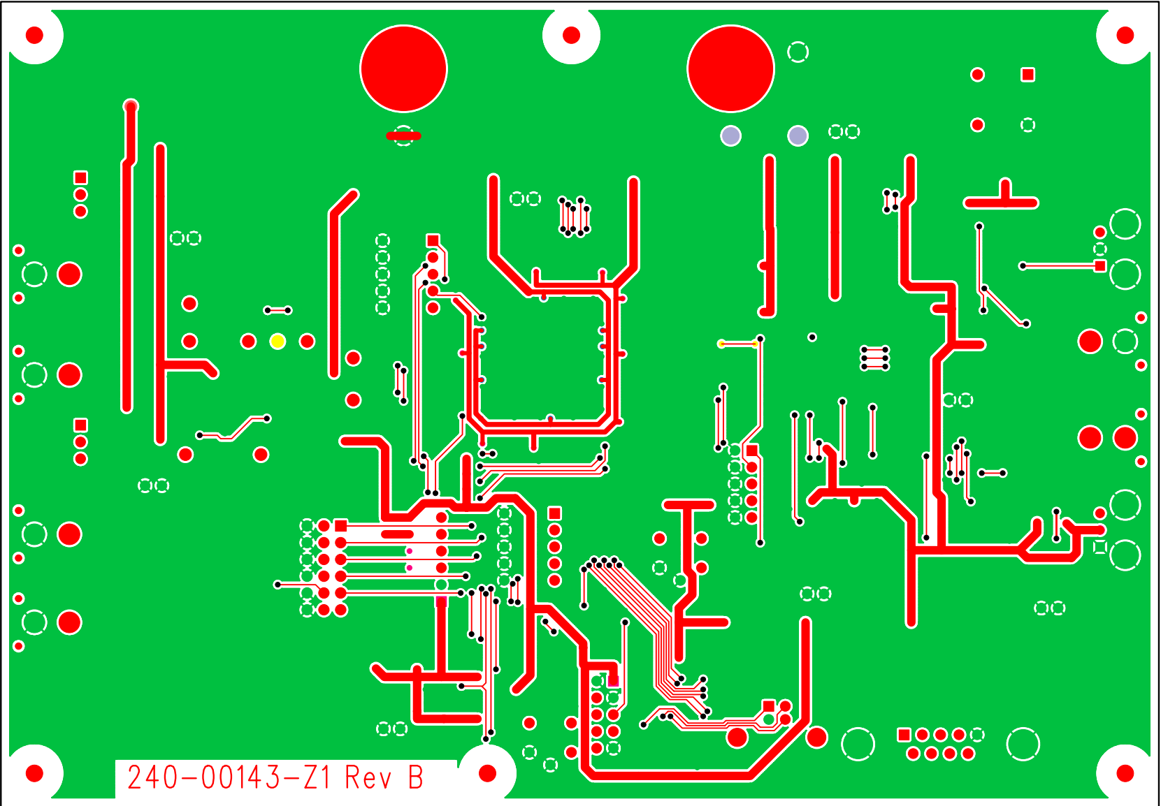
Figure 77. Bottom-Side Layer
