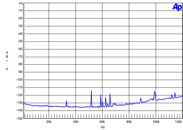
Figure 58. FFT (192 kHz Out-of-Band, No Input)
